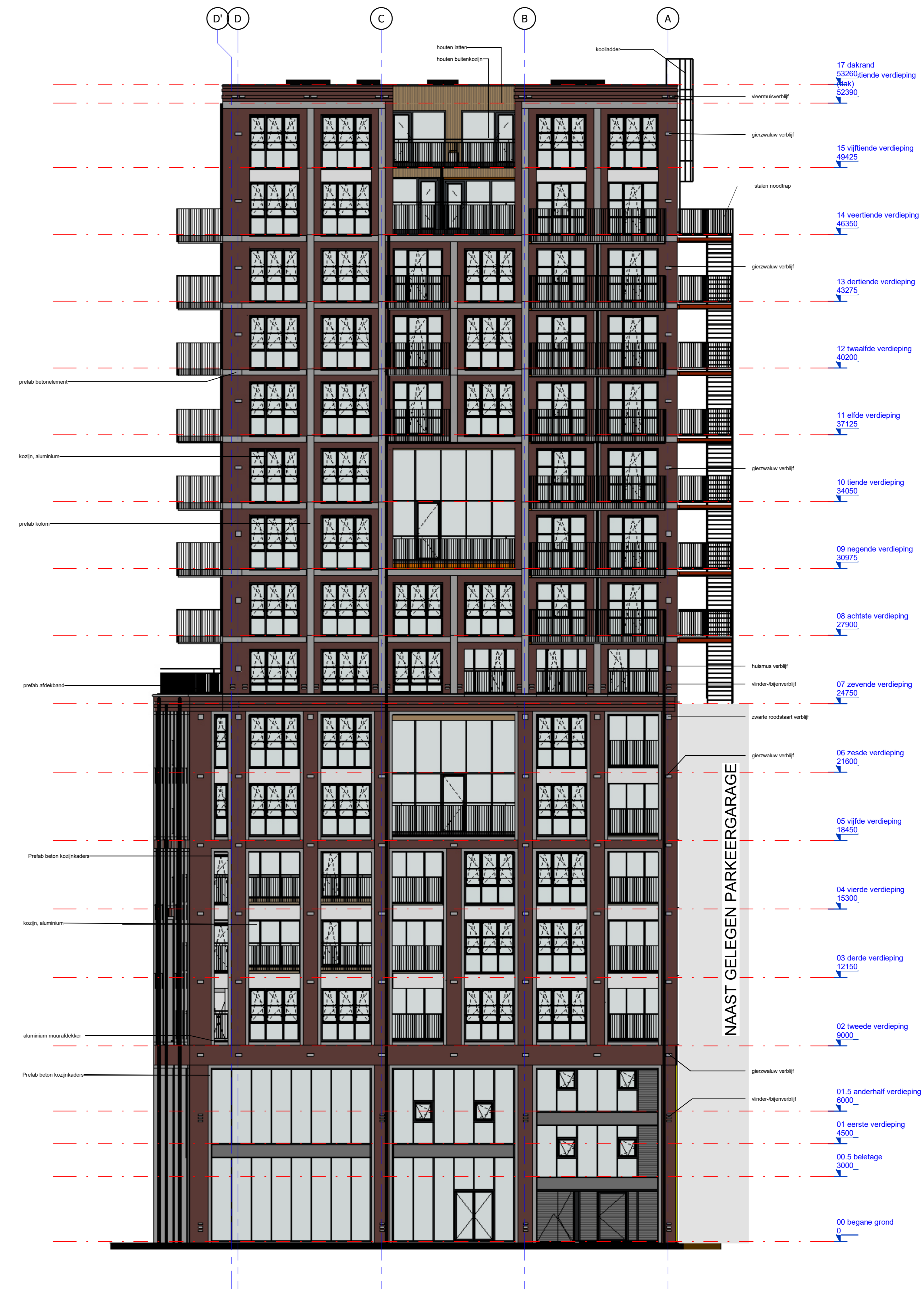
ZO-Gevel (as-6)
